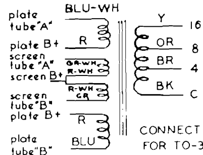
CONNECTIONS FOR "300" SERIES
