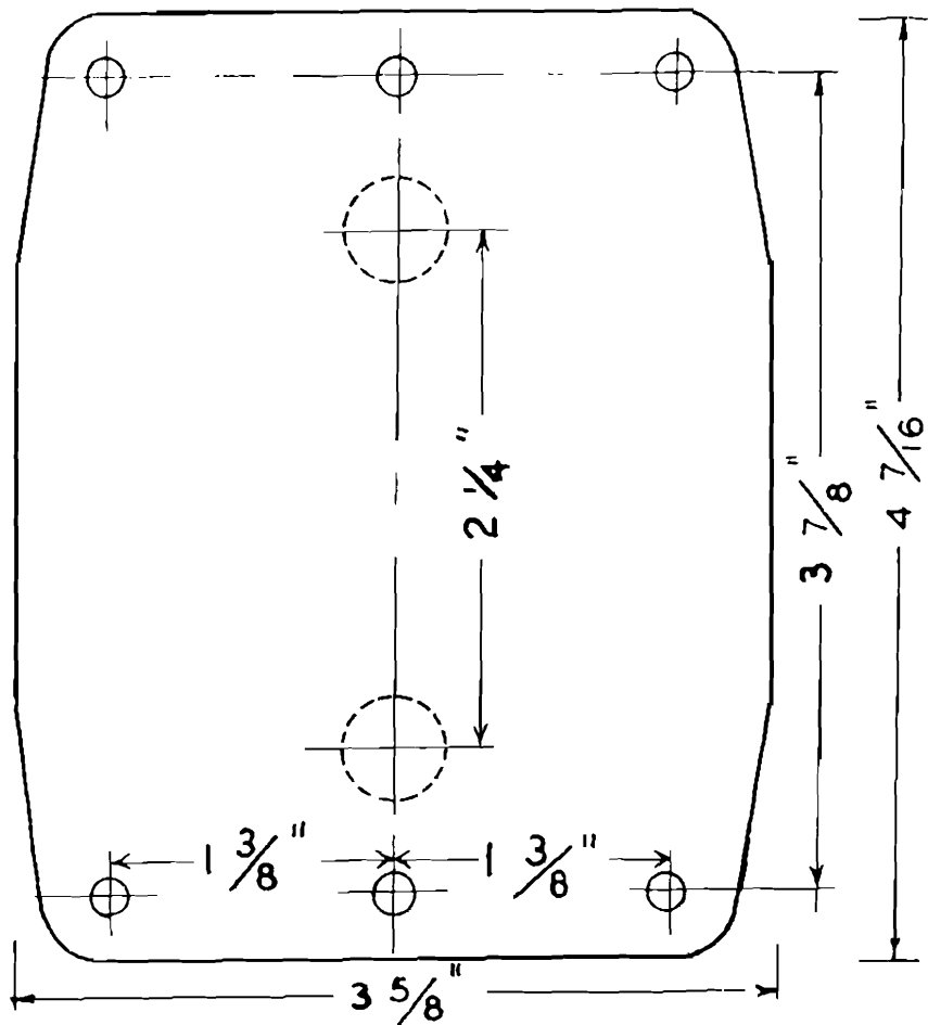
MODELS IN TYPE "A" CASE
